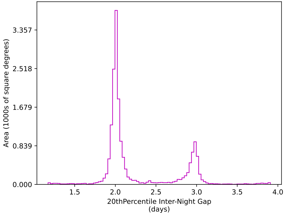
weather_cloudso31v3.4_10yrs WFD z band: 20thPercentile Inter-Night Gap
