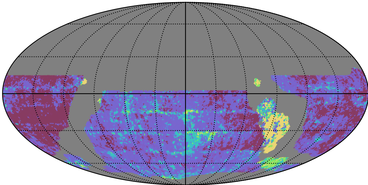
weather_cloudso31v3.4_10yrs WFD y band: 20thPercentile Inter-Night Gap
