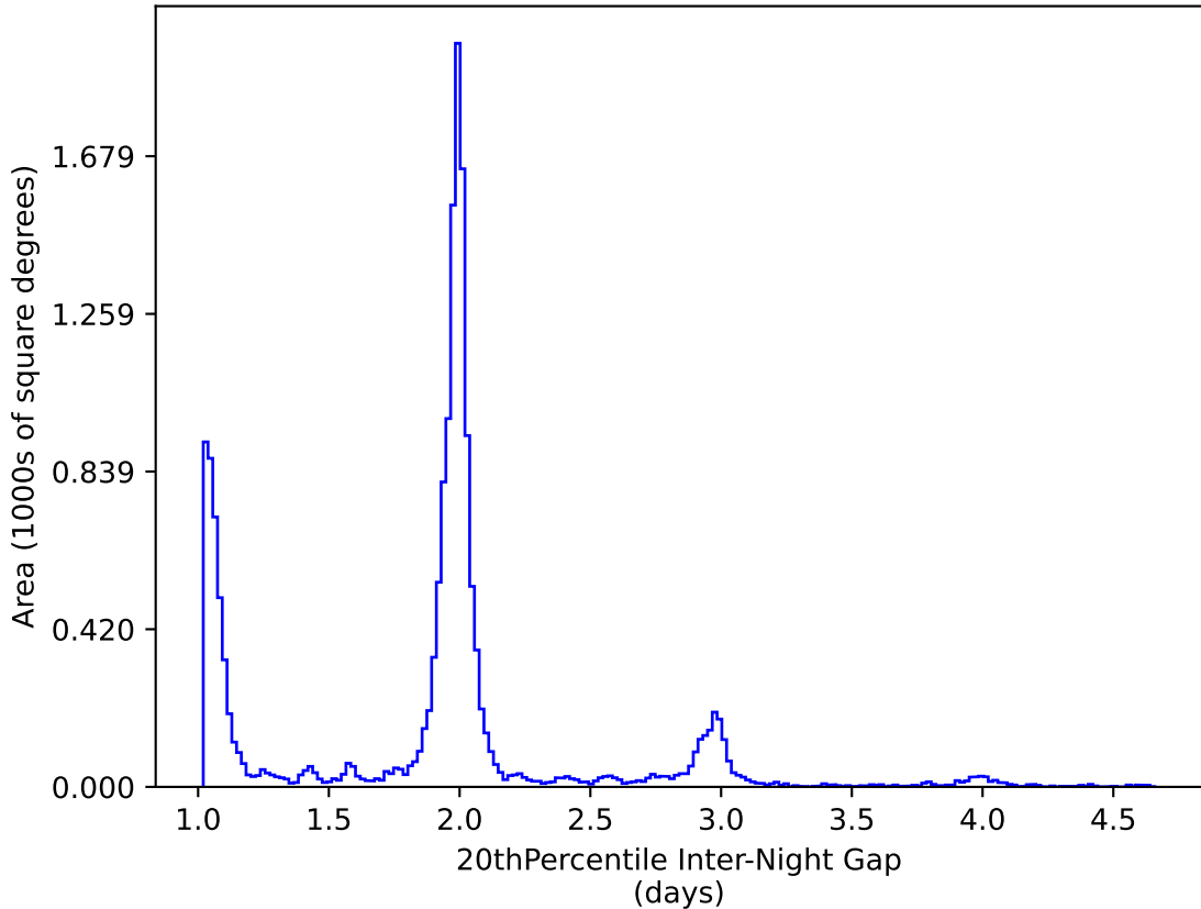
weather_cloudso31v3.4_10yrs WFD y band: 20thPercentile Inter-Night Gap
