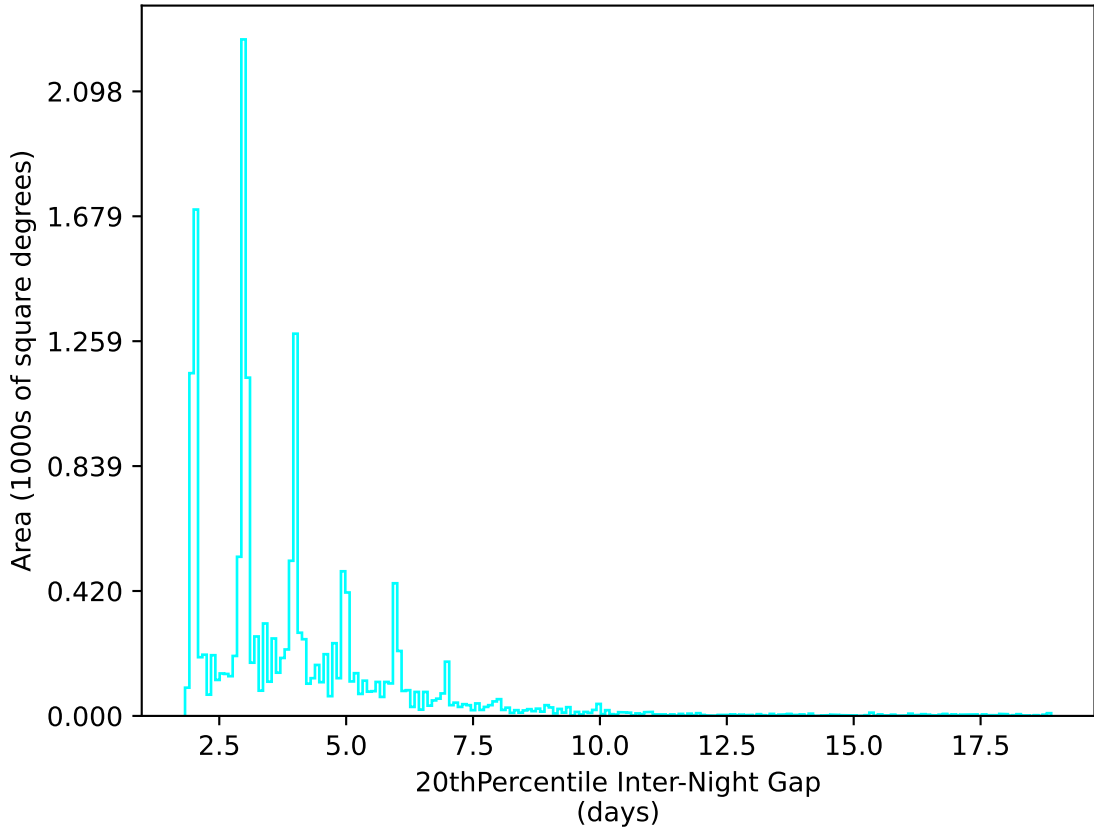
weather_cloudso31v3.4_10yrs WFD u band: 20thPercentile Inter-Night Gap
