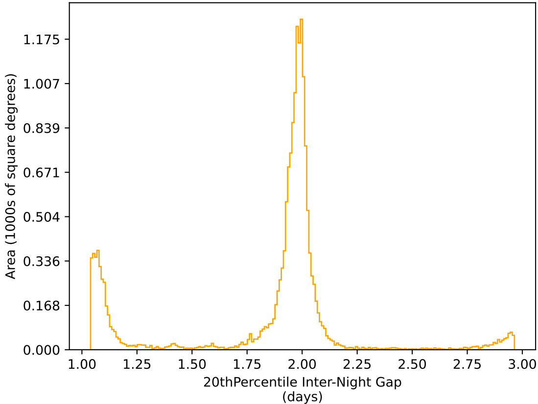
weather_cloudso31v3.4_10yrs WFD r band: 20thPercentile Inter-Night Gap
