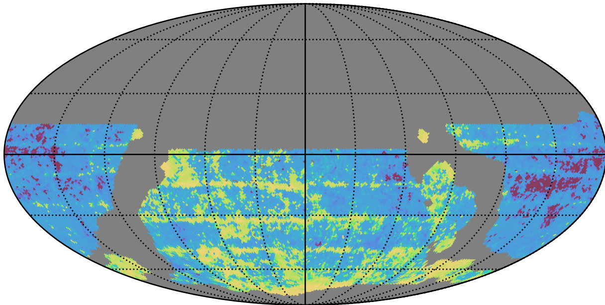
weather_cloudso31v3.4_10yrs WFD i band: 20thPercentile Inter-Night Gap
