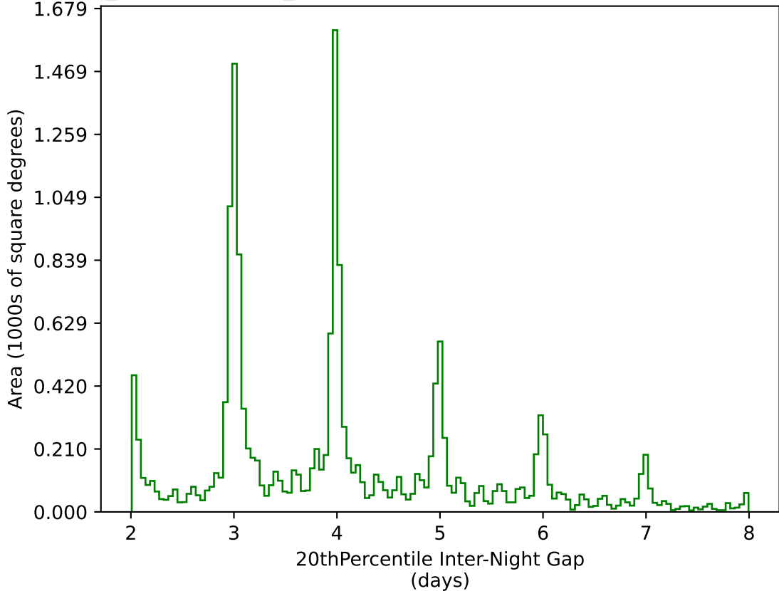
weather_cloudso31v3.4_10yrs WFD g band: 20thPercentile Inter-Night Gap
