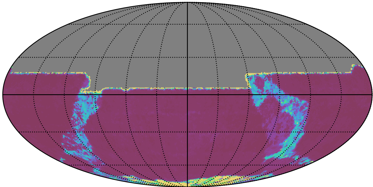
weather_cloudso31v3.4_10yrs All sky y band: 20thPercentile Inter-Night Gap
