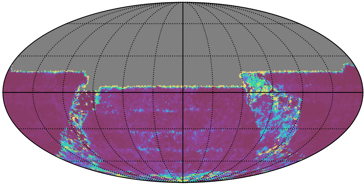
weather_cloudso31v3.4_10yrs All sky u band: 20thPercentile Inter-Night Gap
