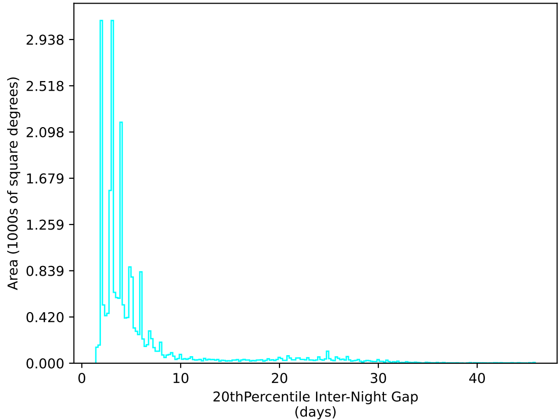
weather_cloudso31v3.4_10yrs All sky u band: 20thPercentile Inter-Night Gap
