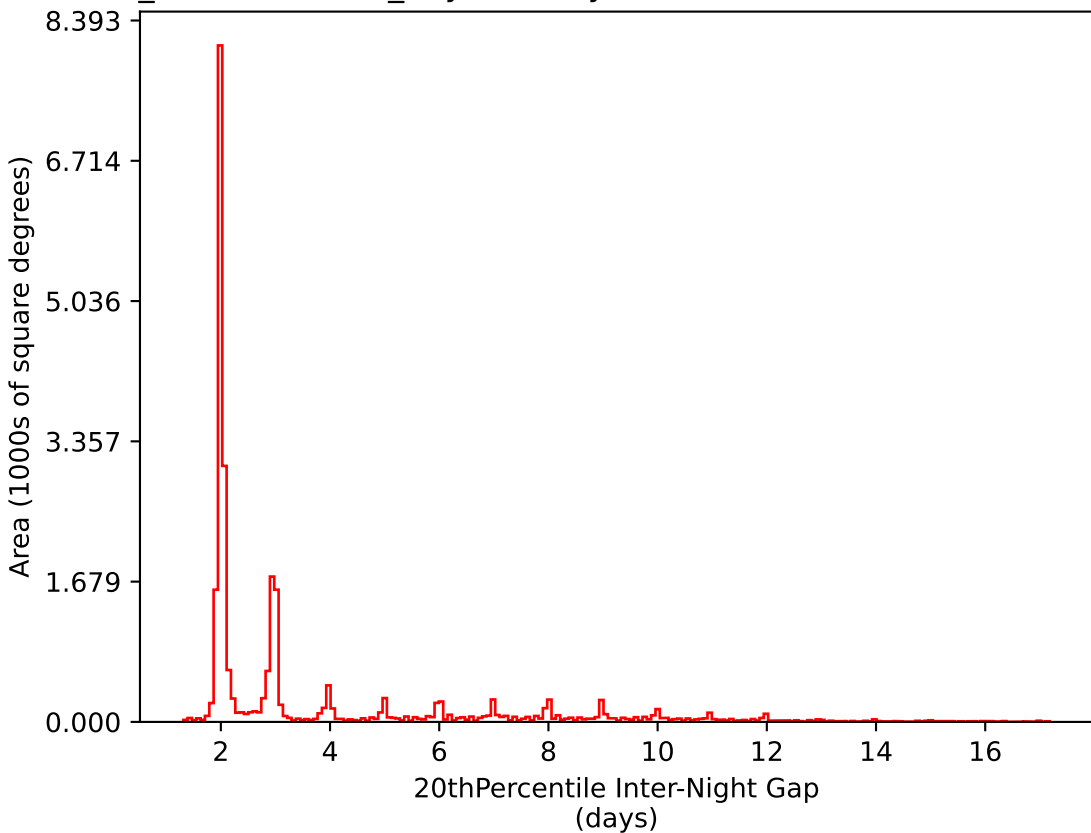
weather_cloudso31v3.4_10yrs All sky i band: 20thPercentile Inter-Night Gap
