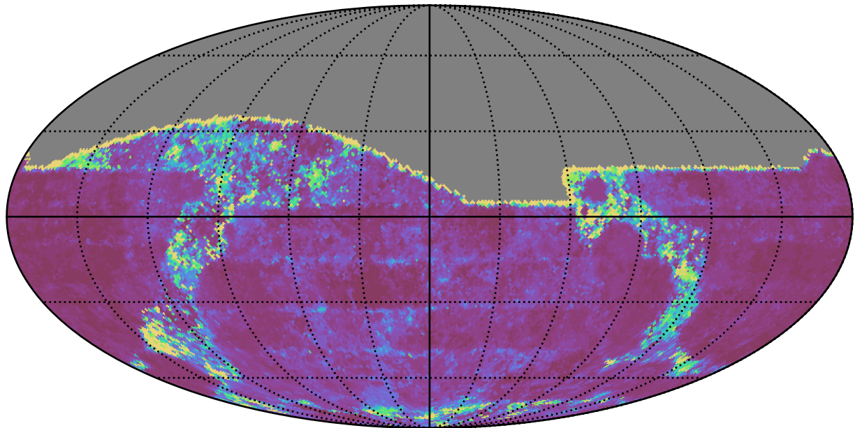
weather_cloudso31v3.4_10yrs All sky g band: 20thPercentile Inter-Night Gap
