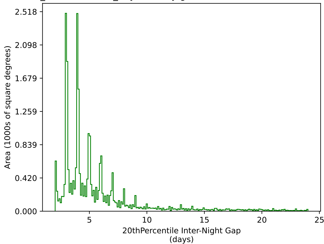
weather_cloudso31v3.4_10yrs All sky g band: 20thPercentile Inter-Night Gap
