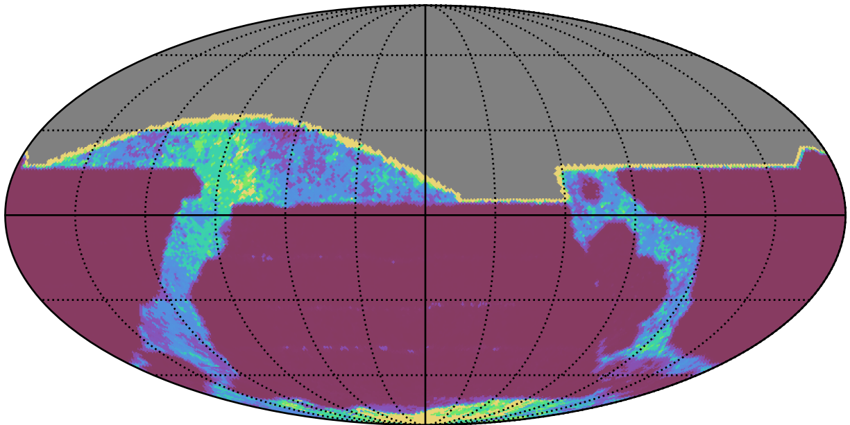
weather_cloudso31v3.4_10yrs All sky all bands: 20thPercentile Inter-Night Gap
