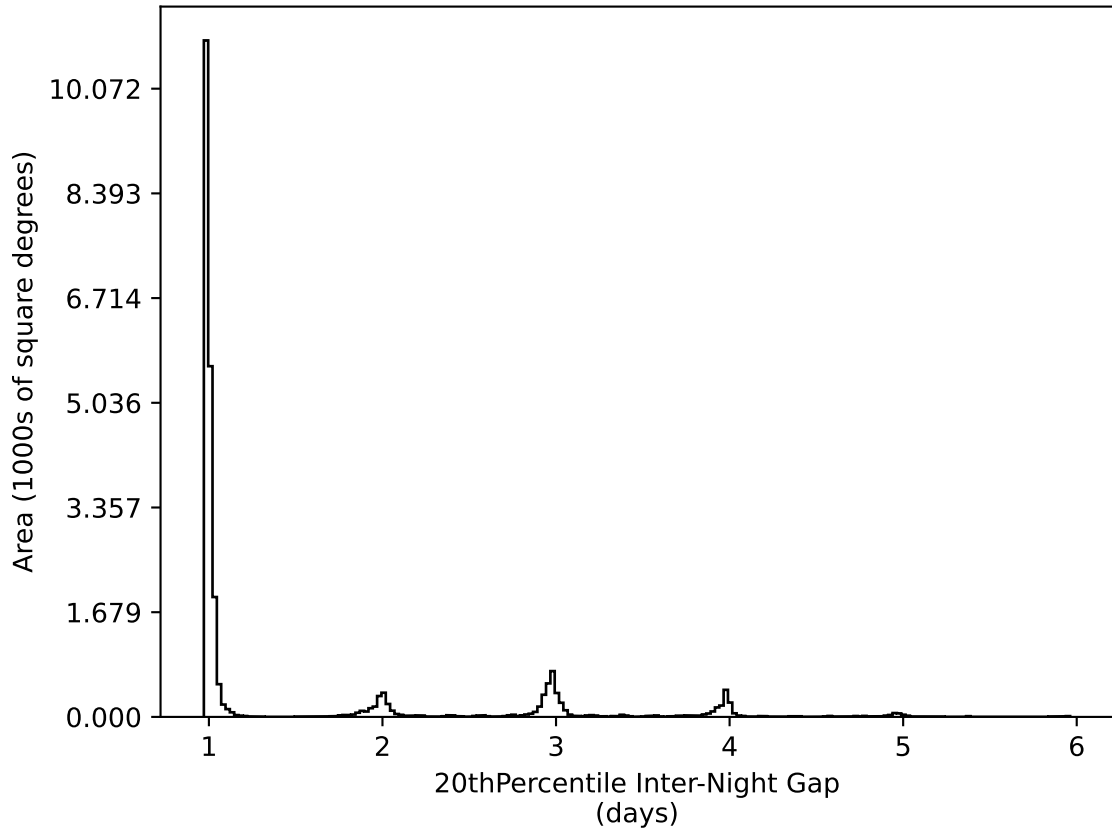
weather_cloudso31v3.4_10yrs All sky all bands: 20thPercentile Inter-Night Gap
