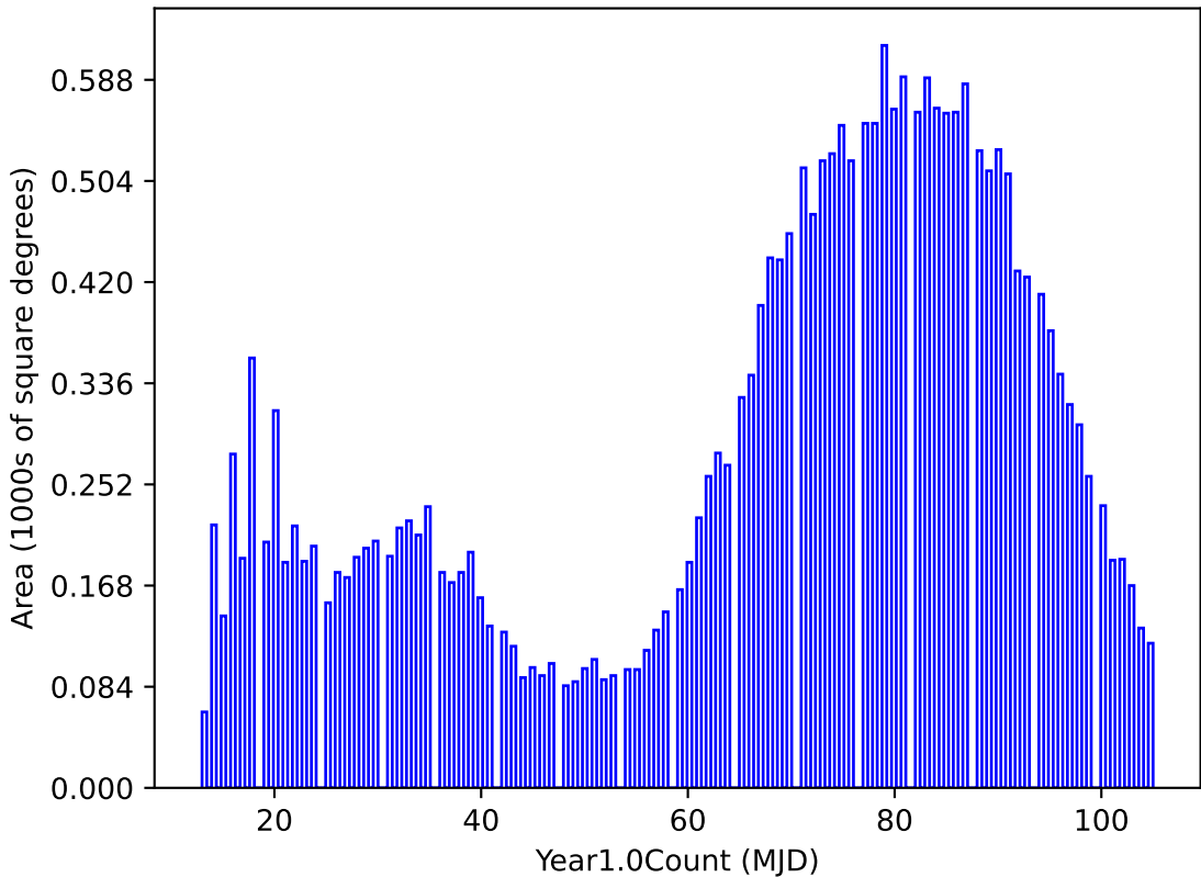
weather_cloudso31v3.4_10yrs night < 365.25: Year1.0Count
