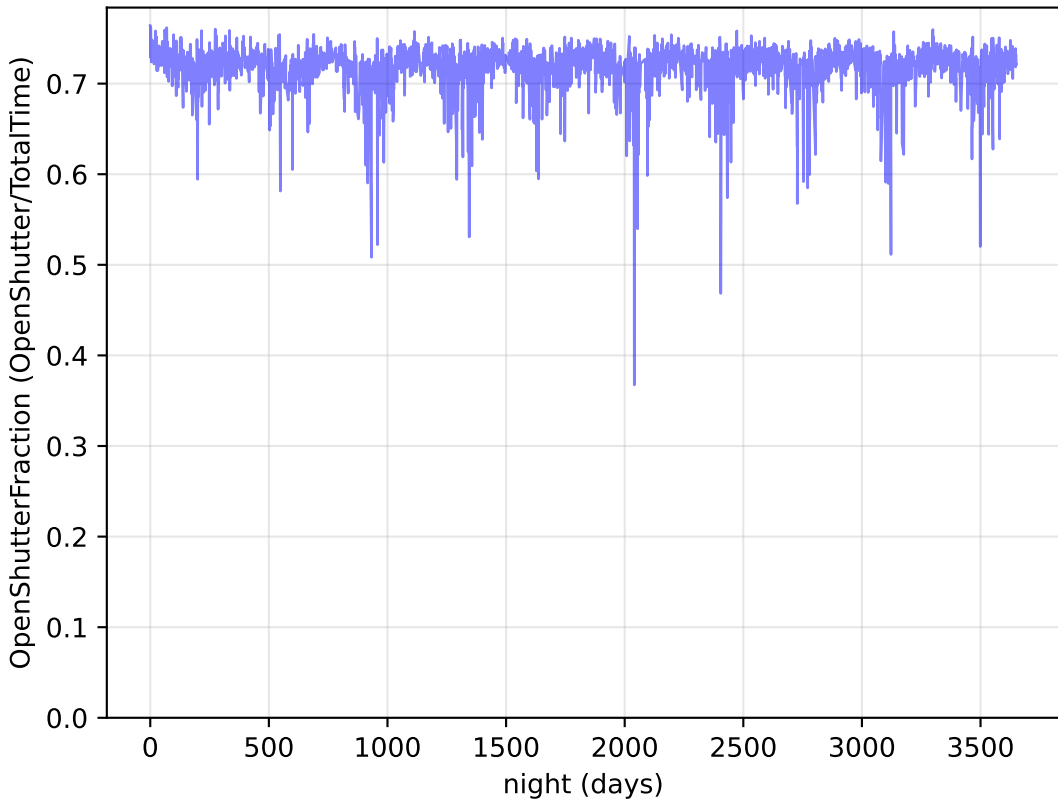
weather_cloudso31v3.4_10yrs : OpenShutterFraction
