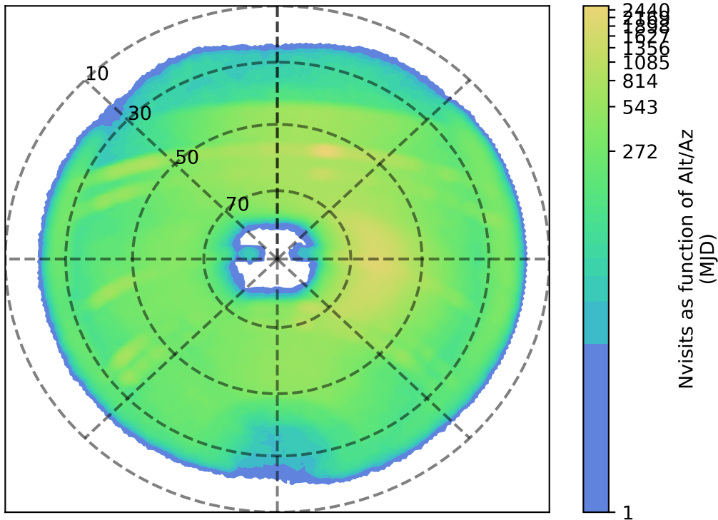
weather_cloudso31v3.4_10yrs z: Nvisits as function of Alt/Az
