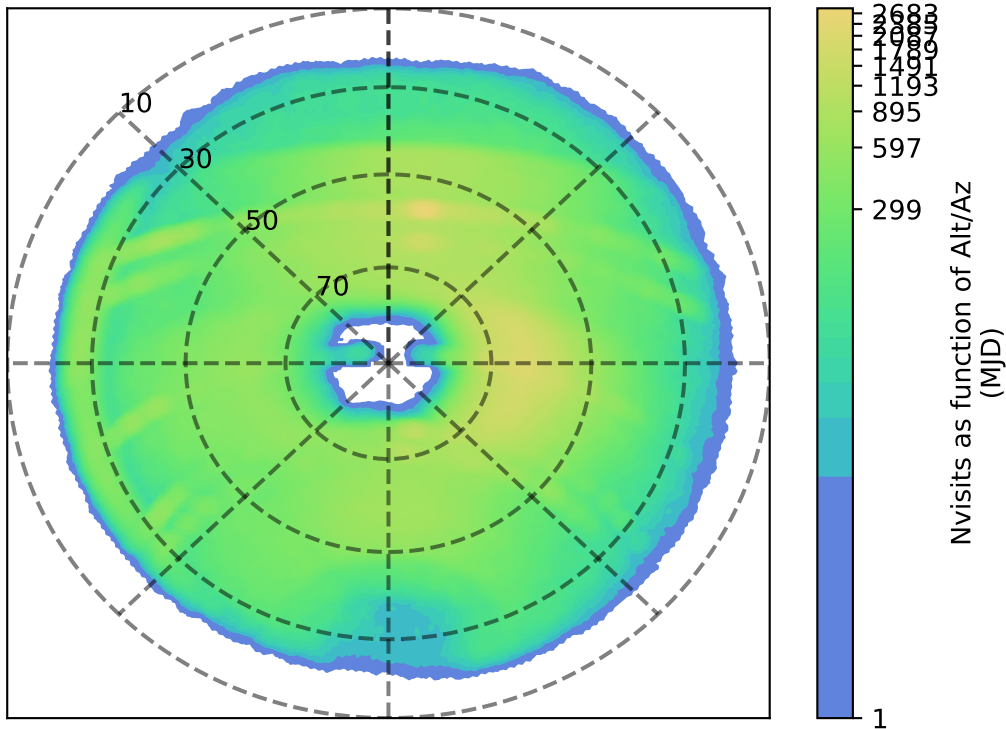
weather_cloudso31v3.4_10yrs r: Nvisits as function of Alt/Az
