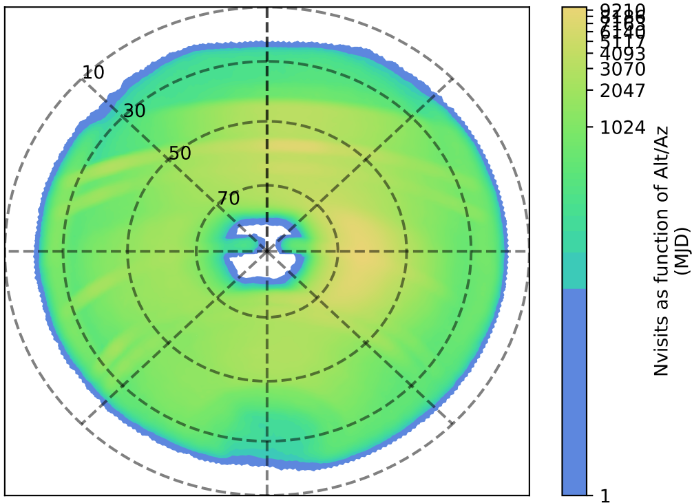
weather_cloudso31v3.4_10yrs : Nvisits as function of Alt/Az
