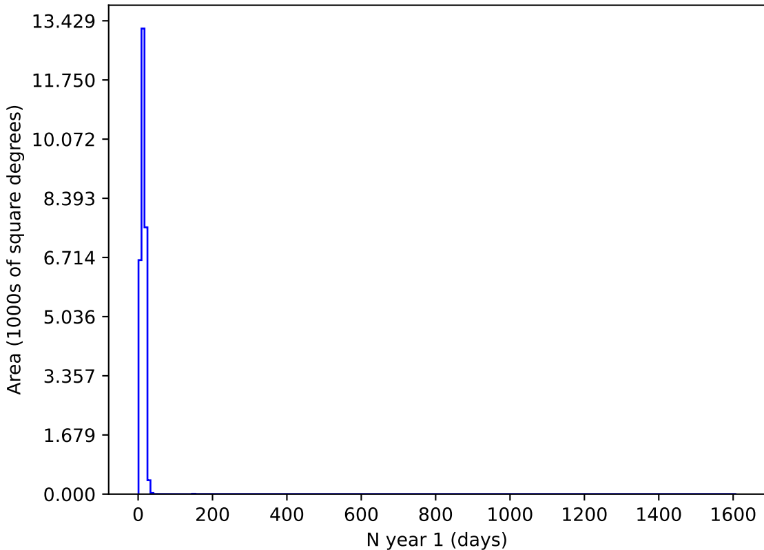
weather_cloudso31v3.4_10yrs r and night < 365: N year 1
