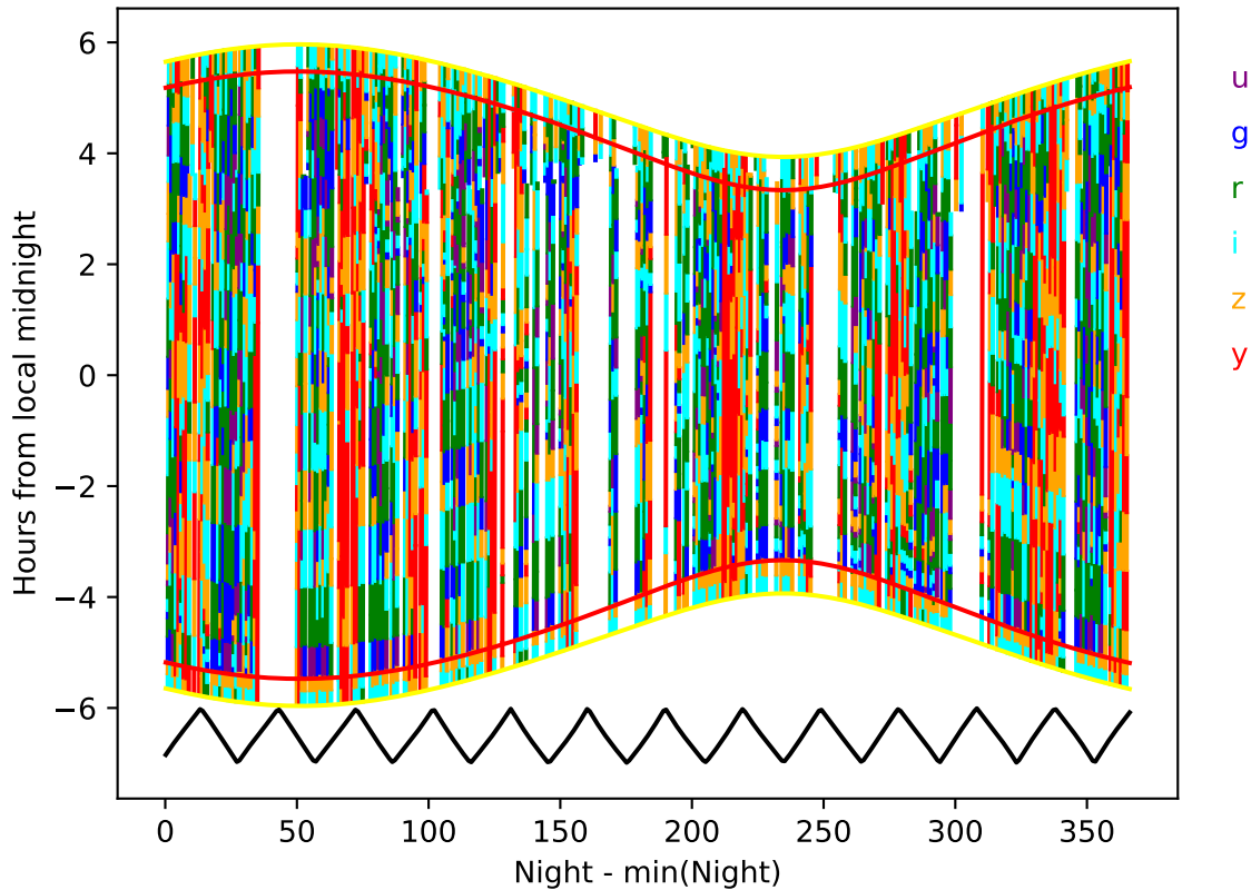
weather_cloudso31v3.4_10yrs year 8-9: Hourglass
