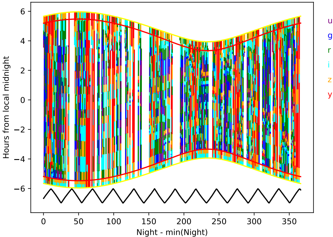
weather_cloudso31v3.4_10yrs year 0-1: Hourglass
