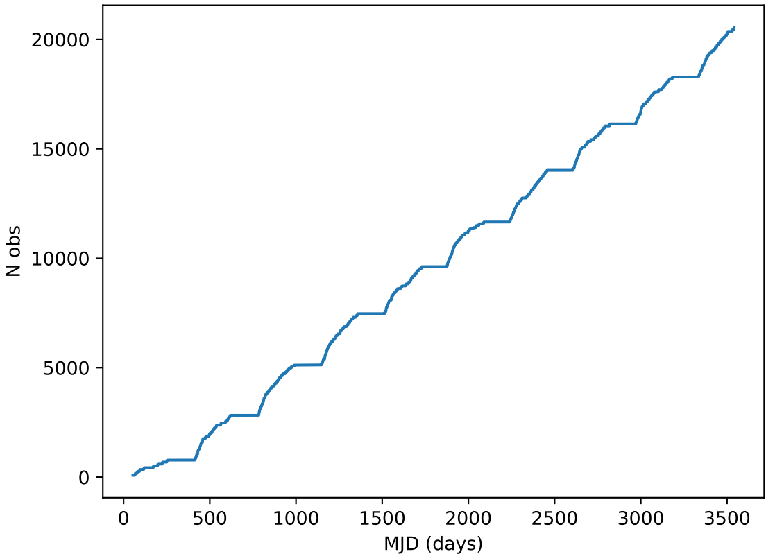
weather_cloudso31v3.4_10yrs note like DD:ELAISS1%: Cumulative
