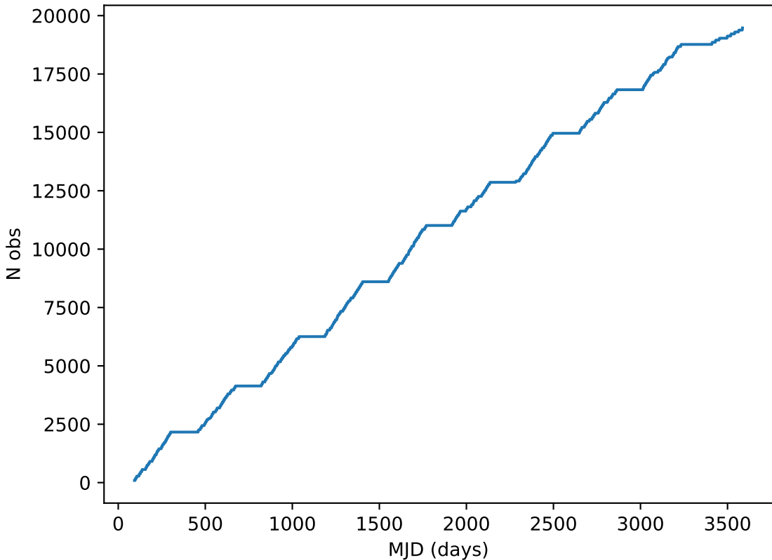
weather_cloudso31v3.4_10yrs note like DD:ECDFS%: Cumulative
