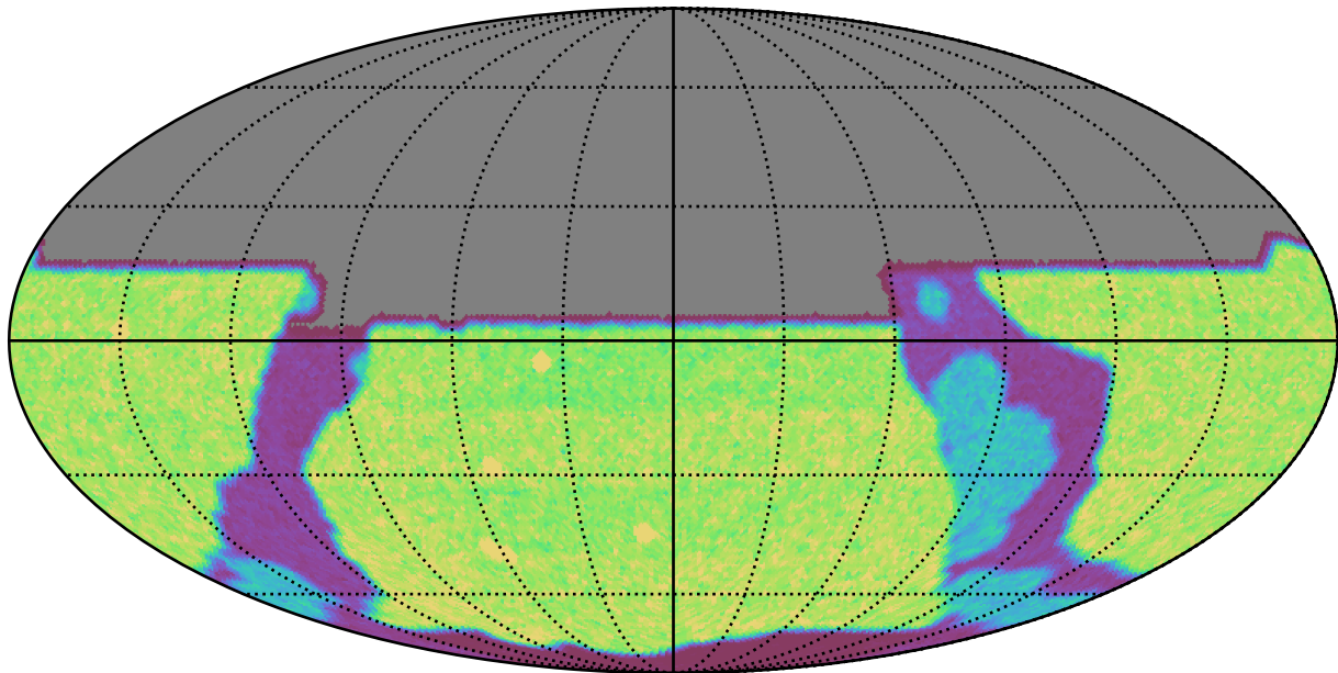
weather_cloudso31v3.4_10yrs y: Count observationStartMJD
