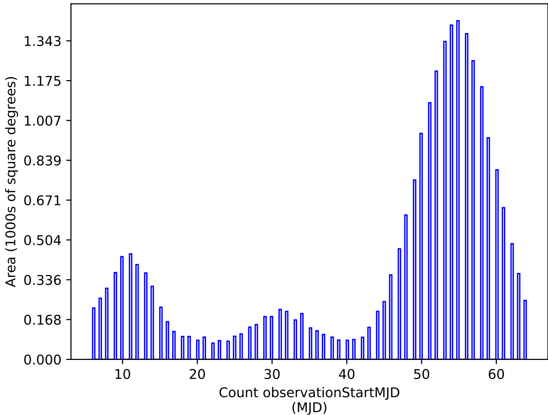
weather_cloudso31v3.4_10yrs u: Count observationStartMJD
