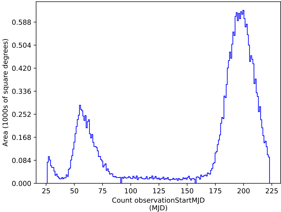
weather_cloudso31v3.4_10yrs i: Count observationStartMJD
