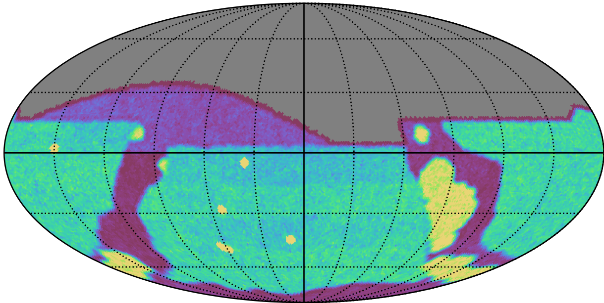
weather_cloudso31v3.4_10yrs g: Count observationStartMJD
