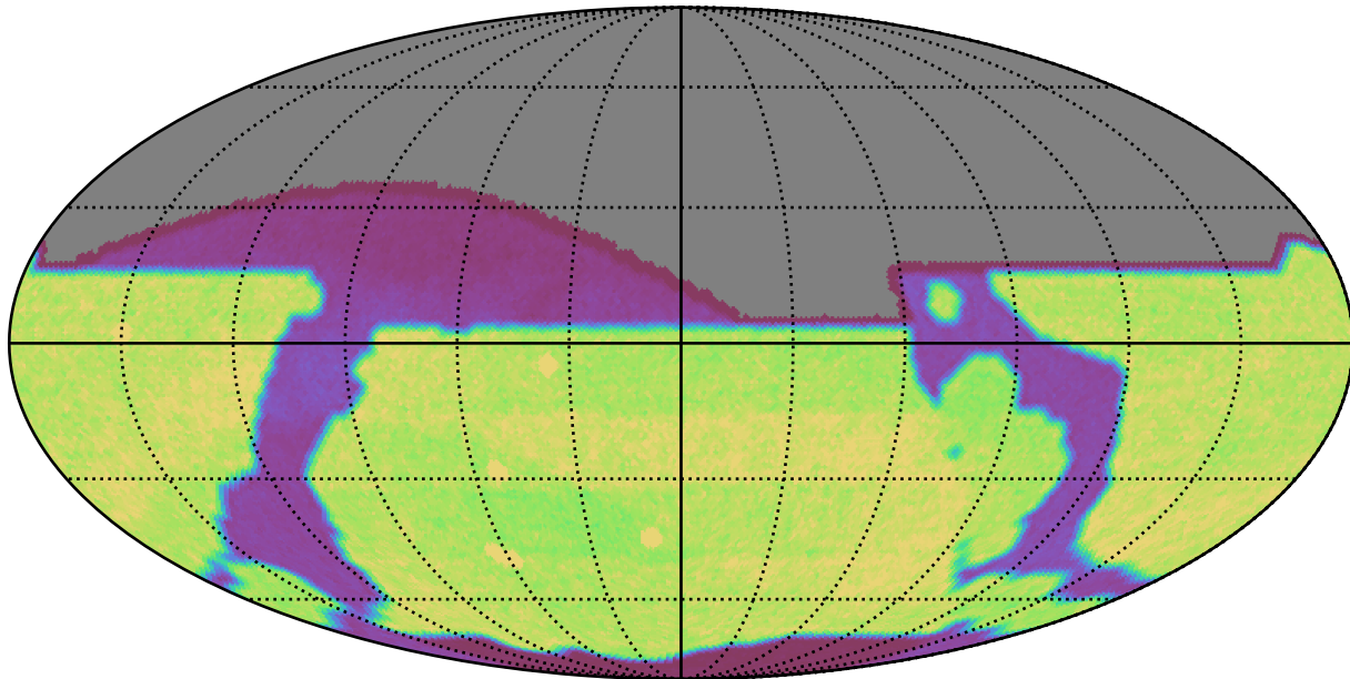
weather_cloudso31v3.4_10yrs : Count observationStartMJD
