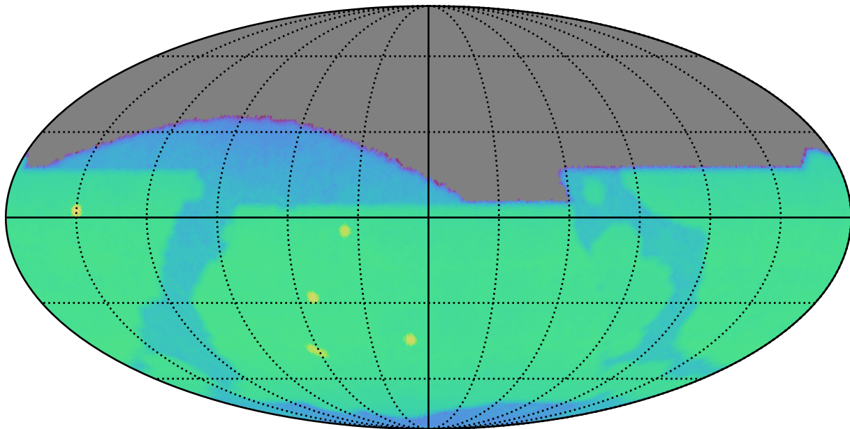
weather_cloudso31v3.4_10yrs z: CoaddM5
