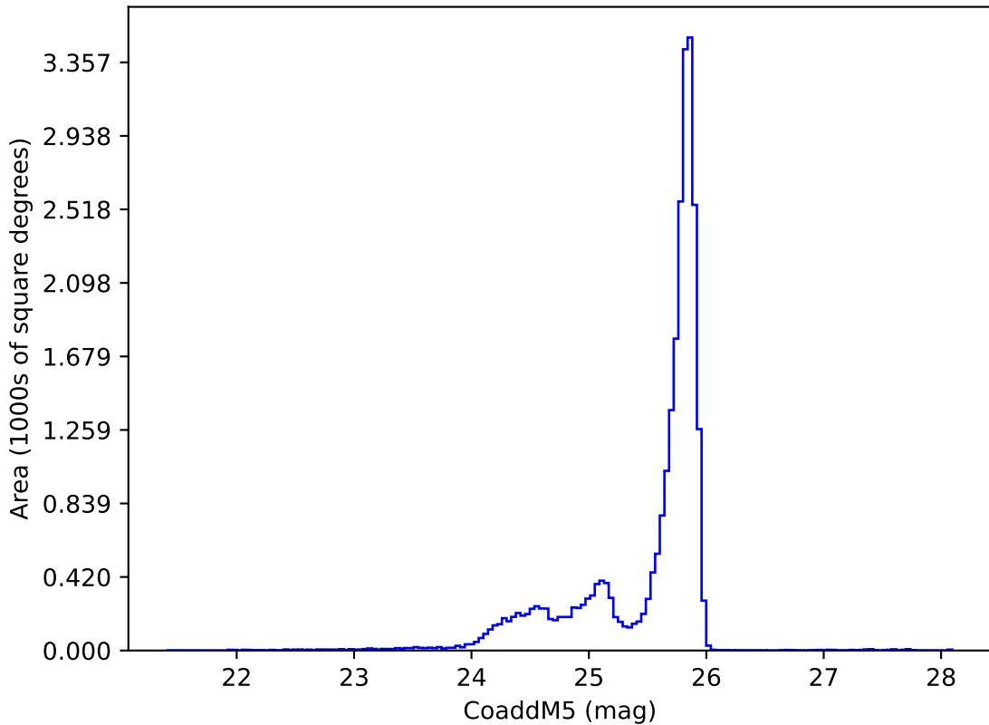
weather_cloudso31v3.4_10yrs z: CoaddM5
