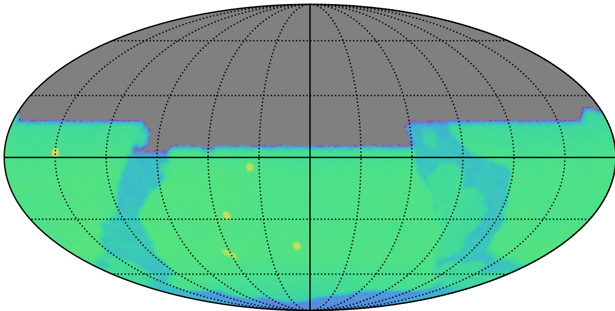
weather_cloudso31v3.4_10yrs y: CoaddM5
