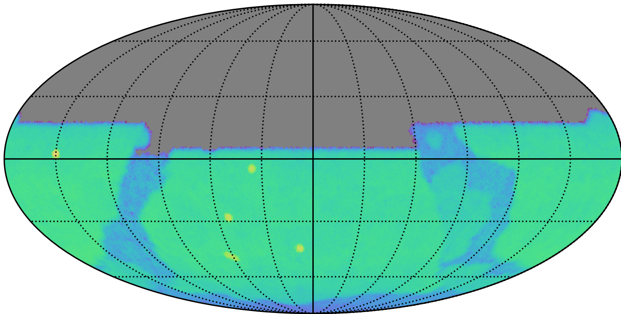
weather_cloudso31v3.4_10yrs u: CoaddM5
