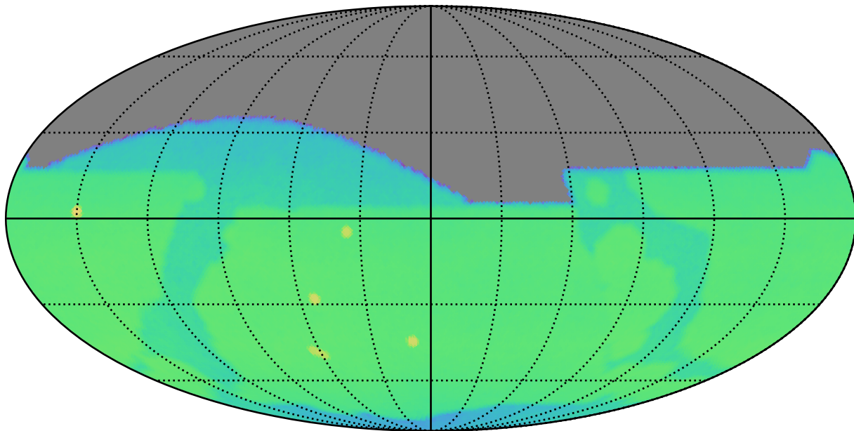
weather_cloudso31v3.4_10yrs r: CoaddM5
