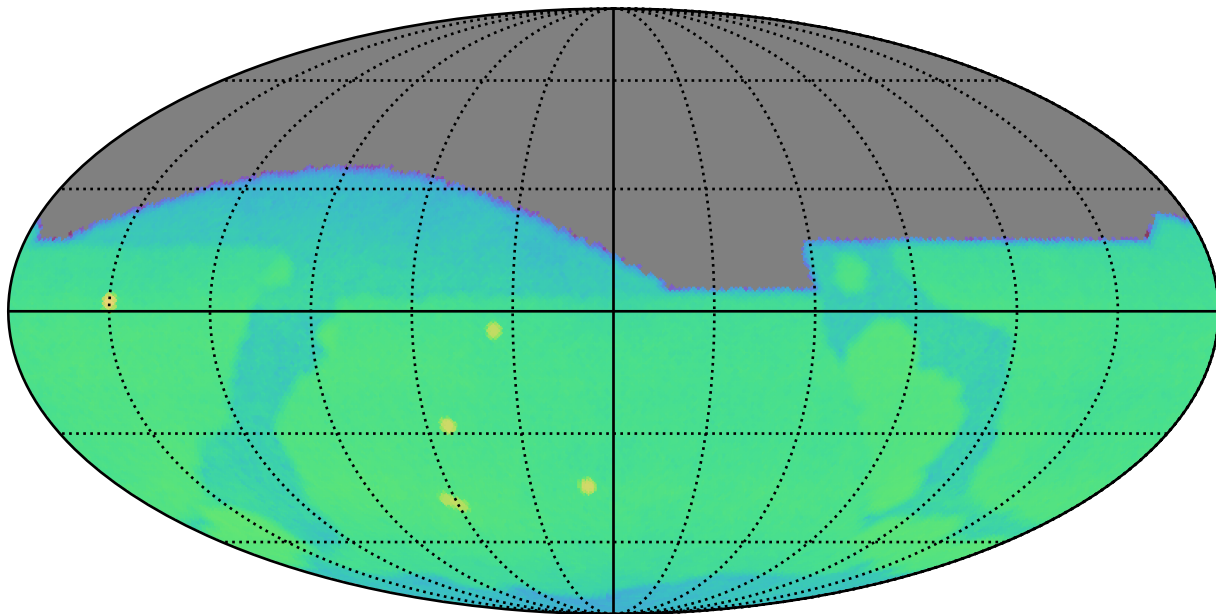
weather_cloudso31v3.4_10yrs g: CoaddM5
