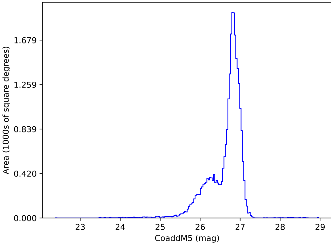
weather_cloudso31v3.4_10yrs g: CoaddM5
