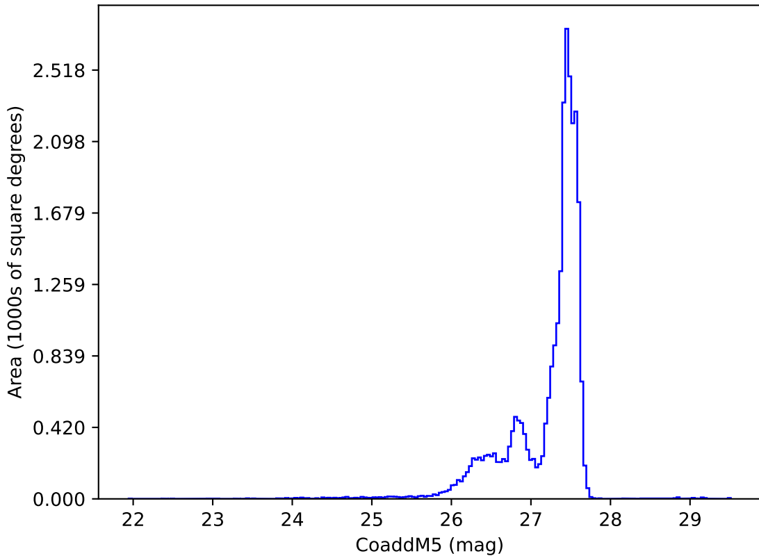
weather_cloudso31v3.4_10yrs : CoaddM5
