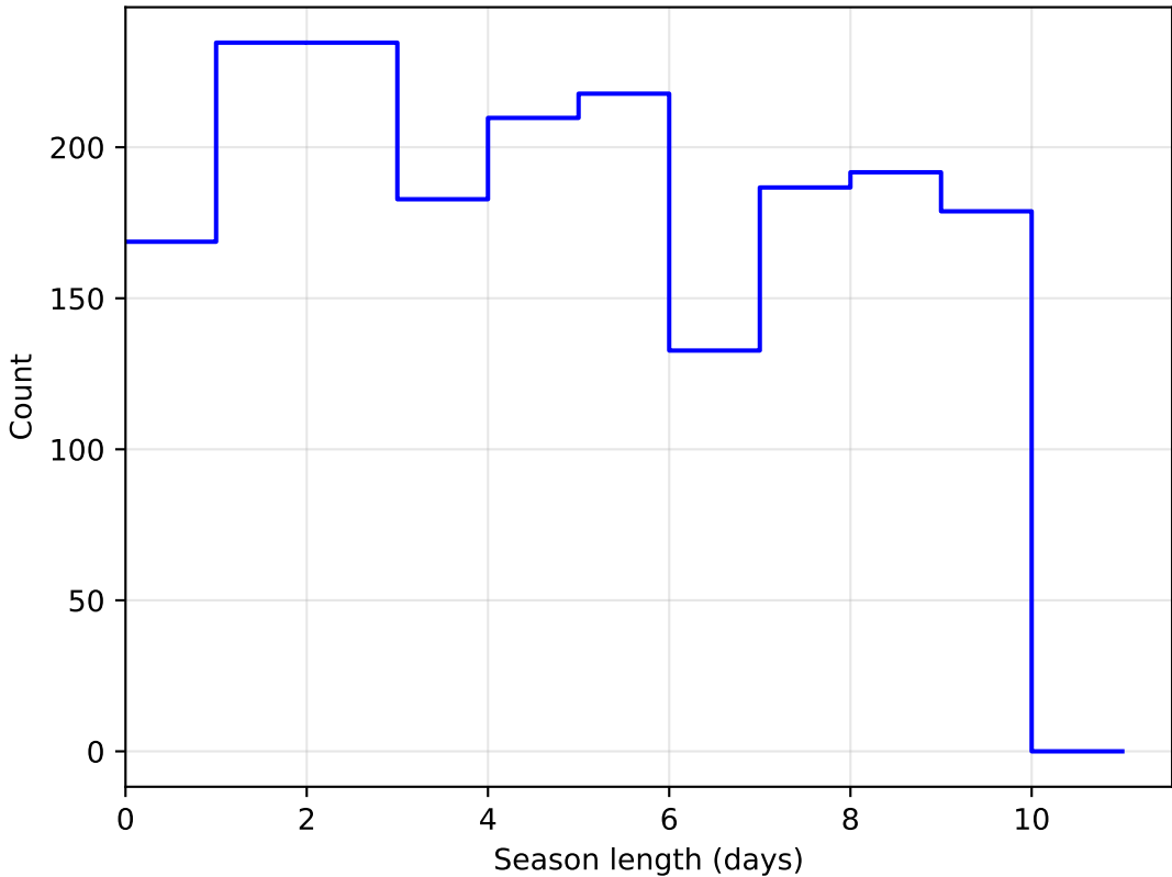
weather_cloudso31v3.4_10yrs DD:WFD all bands: SeasonLength
