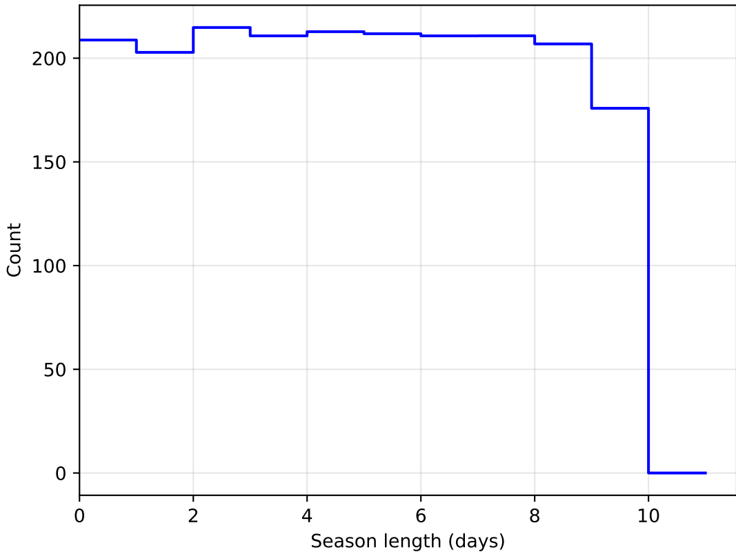
weather_cloudso31v3.4_10yrs DD:EDFS all bands: SeasonLength
