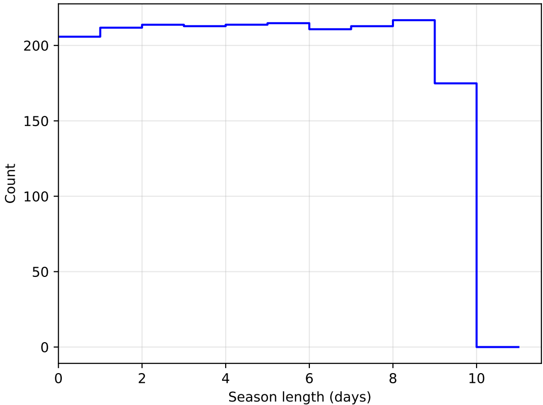
weather_cloudso31v3.4_10yrs DD:ECDFS all bands: SeasonLength
