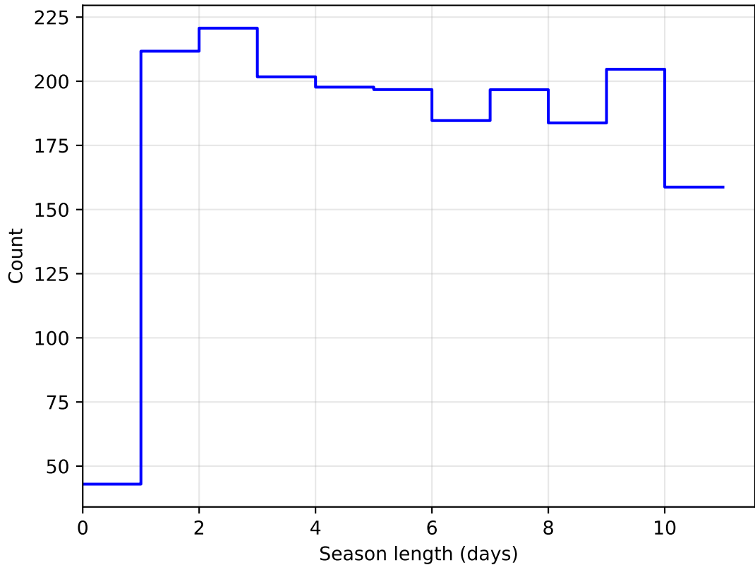
weather_cloudso31v3.4_10yrs DD: COSMOS all bands: SeasonLength
