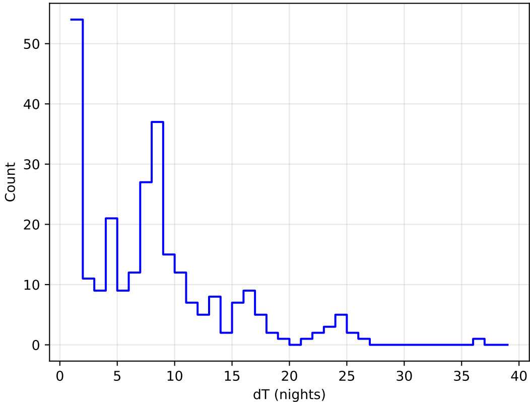
weather_cloudso31v3.4_10yrs all bands: DD:XMM_LSS Delta Nights Histogram
