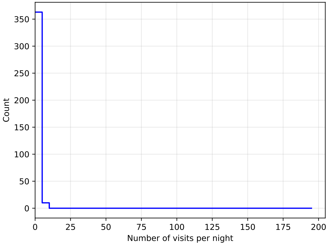
weather_cloudso31v3.4_10yrs all bands: DD:WFD NVisitsPerNight
