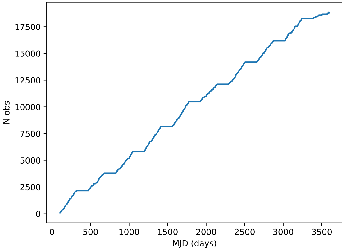
weather_cloudso31v3.4_10yrs all bands: DD:EDFS Cumulative NVisits
