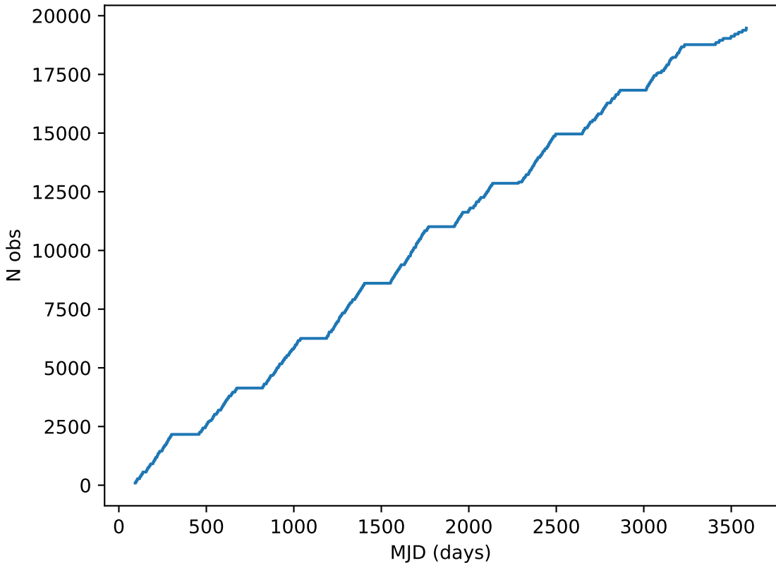
weather_cloudso31v3.4_10yrs all bands: DD:ECDFS Cumulative NVisits
