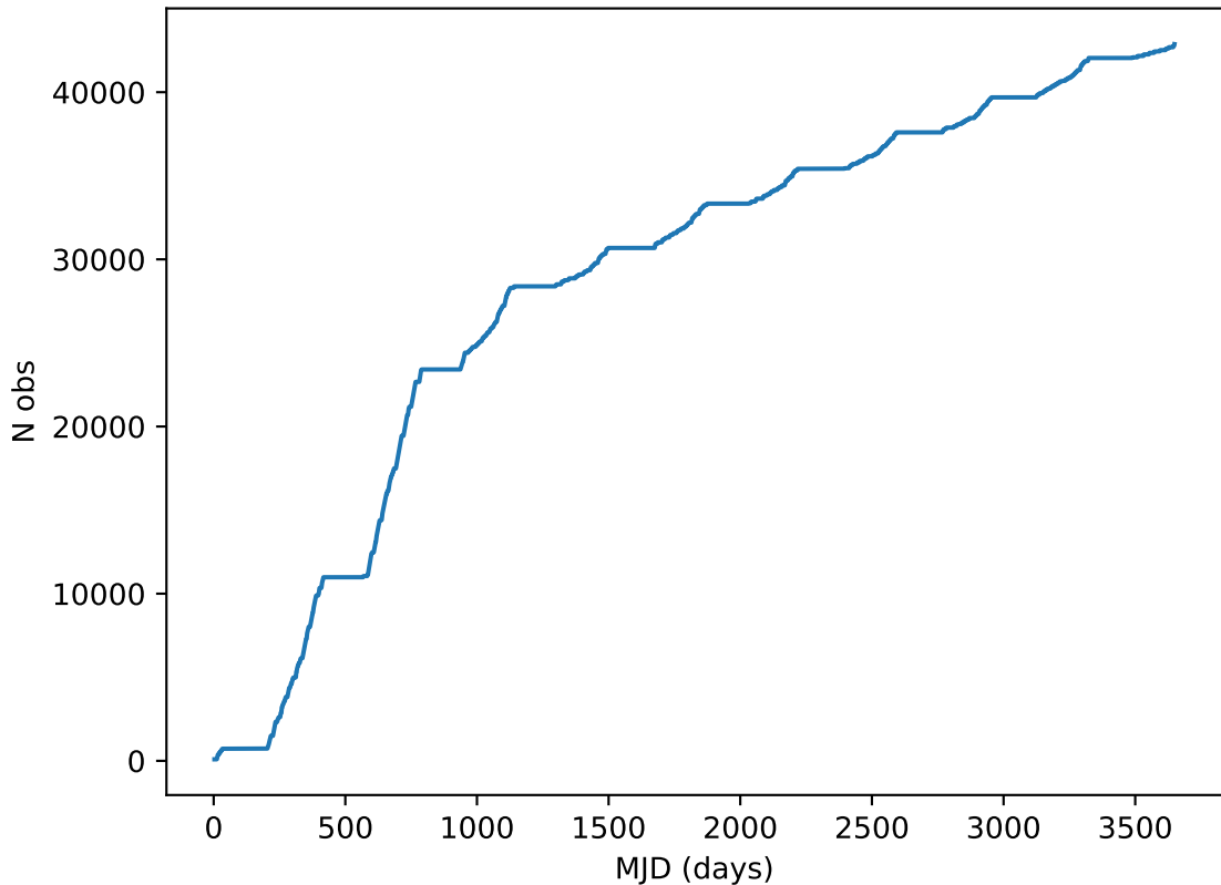
weather_cloudso31v3.4_10yrs all bands: DD:COSMOS Cumulative NVisits
