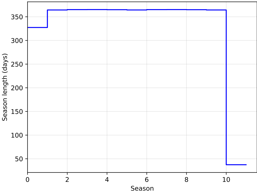
weather_cloudso30v3.5_10yrs DD:WFD all bands: SeasonLength
