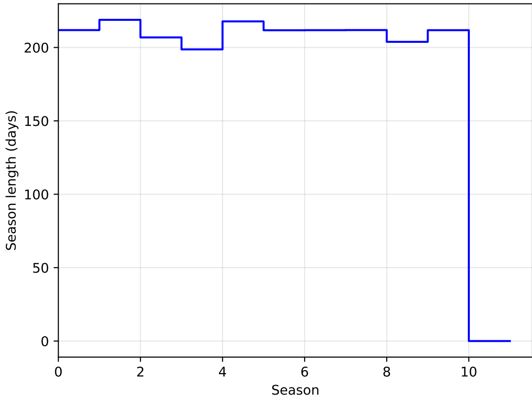
weather_cloudso30v3.5_10yrs DD:ELAISS1 all bands: SeasonLength
