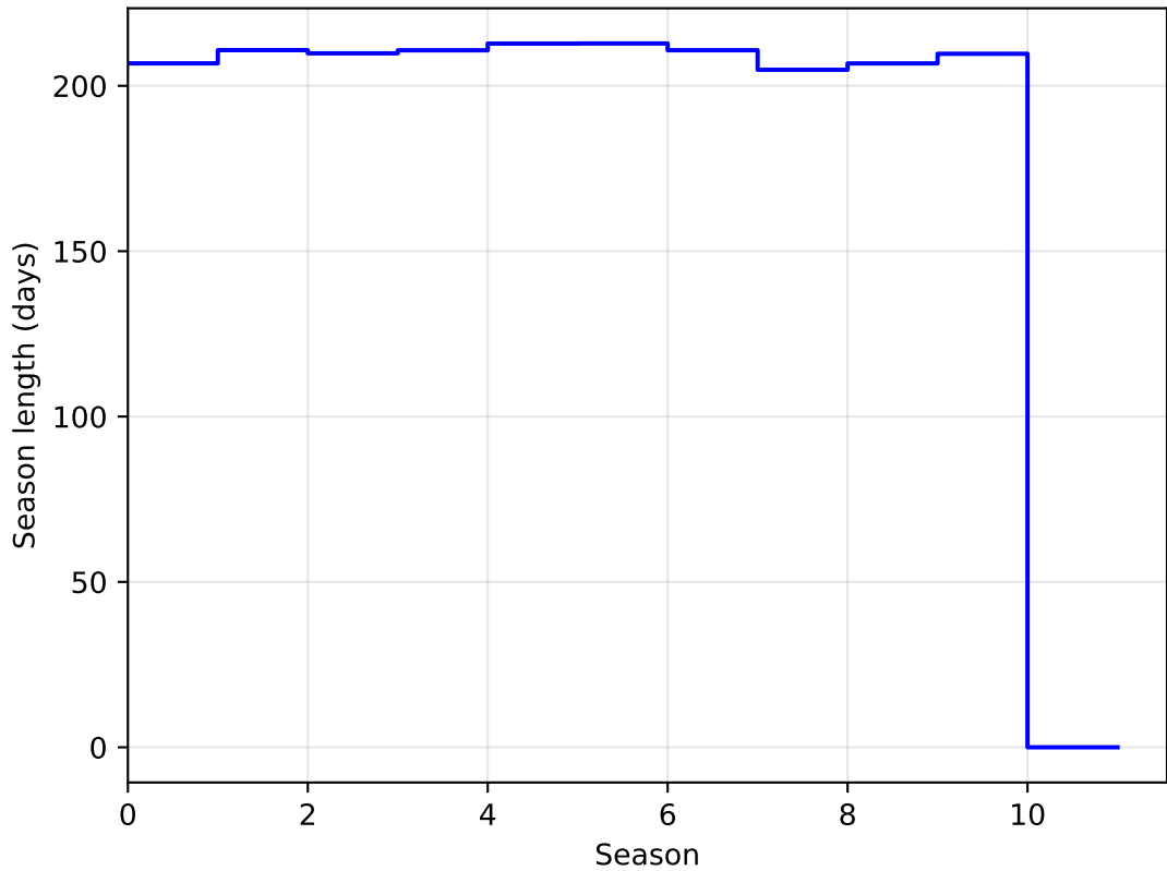
weather_cloudso30v3.5_10yrs DD:EDFS all bands: SeasonLength
